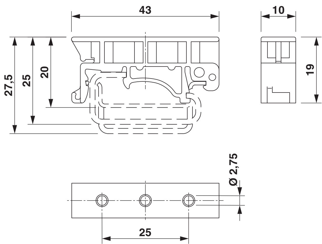
Dimensional drawing
