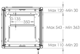
MAX//MIN EQUIPMENT MOUNTING DISTANCE
