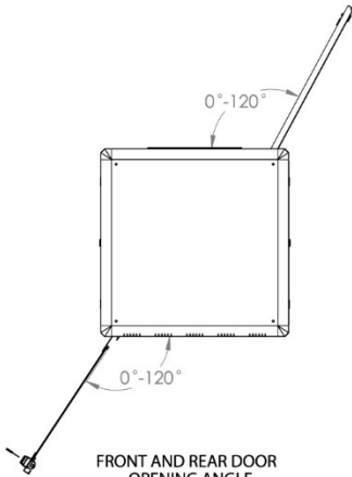
FRONT AND REAR DOOR OPENING ANGLE
